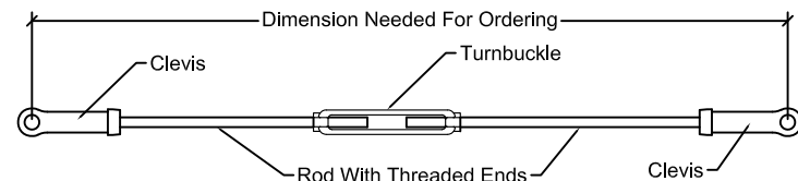
Clevis Assembly With Turnbuckle (Can Be Ordered Without Turnbuckle)
