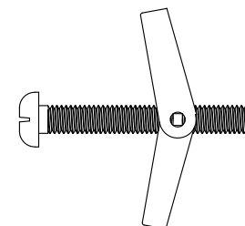
Toggle Bolt Used For Fastening To Drywall Holes to Be \frac{1}{16} " - \frac{1}{8} " Oversized
