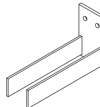
Bottom Saddle Clip Used For Attaching Bottom Rail Of Guardrail To Wall Different Variations Available See Typ. Parts Book
